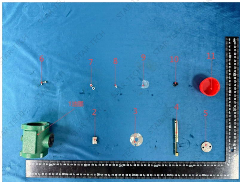
Figure 2. Disassembling photo
